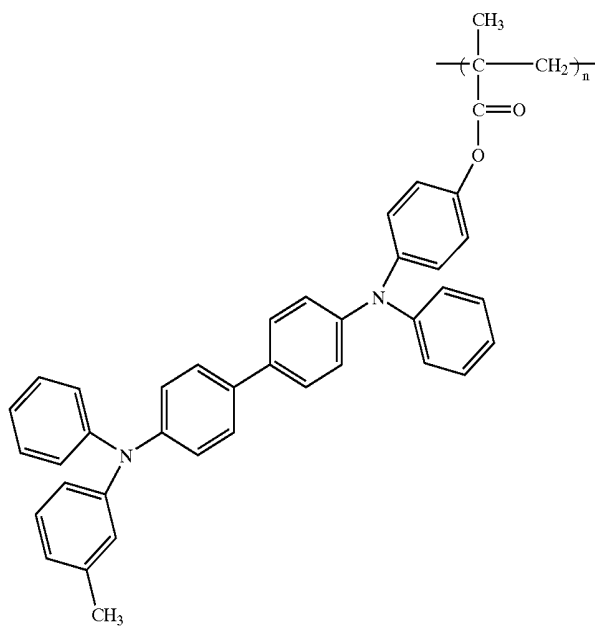
Tpd-PMMA
