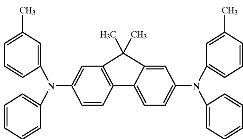
DTDPPFL
