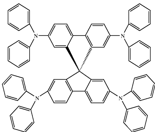
spiro-TPD
